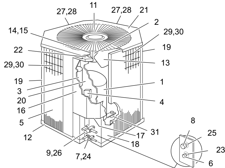
FIGURE 1 -SPLIT SYSTEM, COOLING, OUTDOOR SECTION
