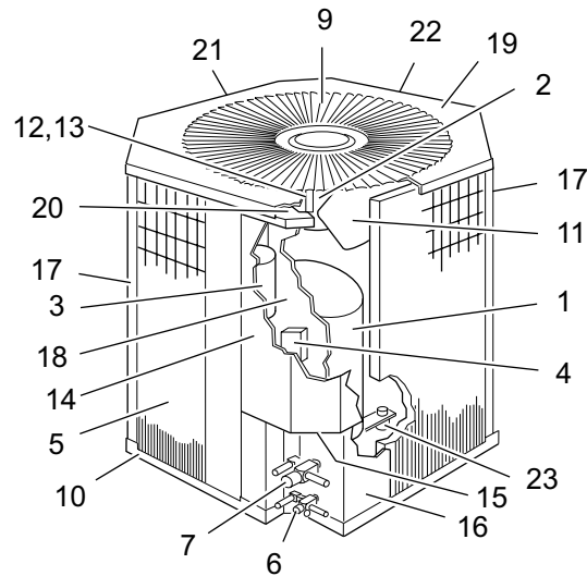
FIGURE 2 -SPLIT SYSTEM, COOLING, OUTDOOR SECTION
