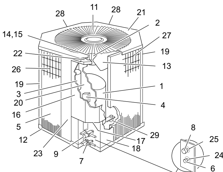
FIGURE 3 - SPLIT SYSTEM, COOLING, OUTDOOR SECTION
