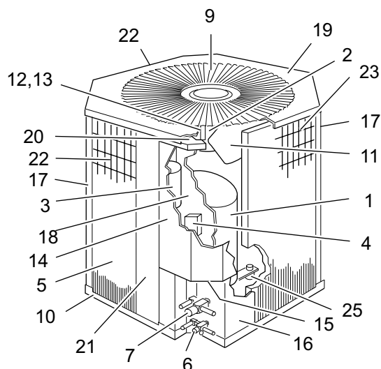
FIGURE 4 - SPLIT SYSTEM, COOLING, OUTDOOR SECTION
